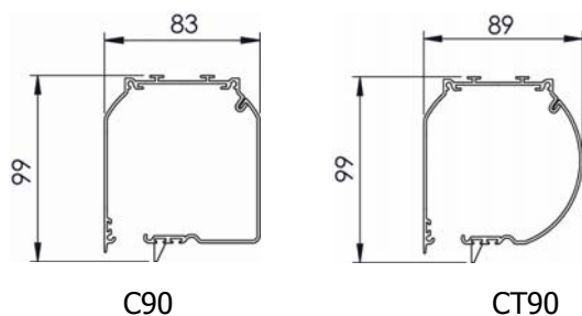
Dimensioni in mm Dimensions shown in mm
